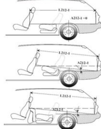
PART 3 – Description of the Package Drawing and Dimension List FIGURE 26-2: LUGGAGE FLOOR LENGTH – FIRST L212-1, A212-1
